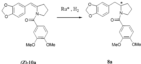
Scheme 4. Enantioselective hydrogenation of (Z)- 10a
