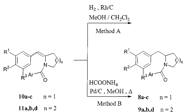
Scheme 3. Synthesis of 1-aryl- and -heteroaroyl-2-arylmethylpyrrolidines and -piperidines
