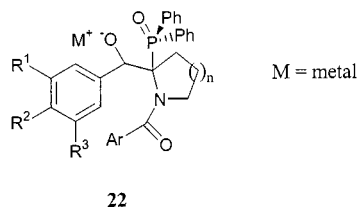
Figure 2. Primary adduct of the Horner reaction
