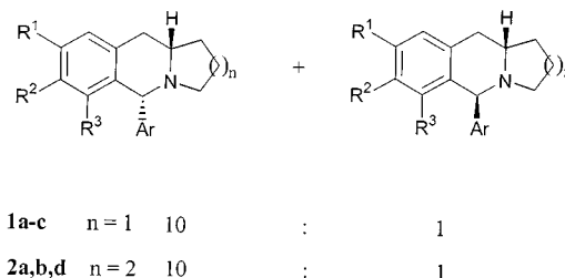
Scheme 5. Synthesis of 5-(or-6)-arylbenzoindolizidines and -quinoxalidines
