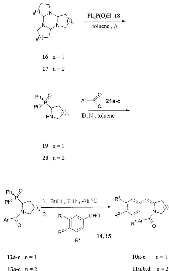
Scheme 2. Synthesis of 1-aryl- and -heteroaryl-2-arylmethylenepyrrolidines and -piperidines
